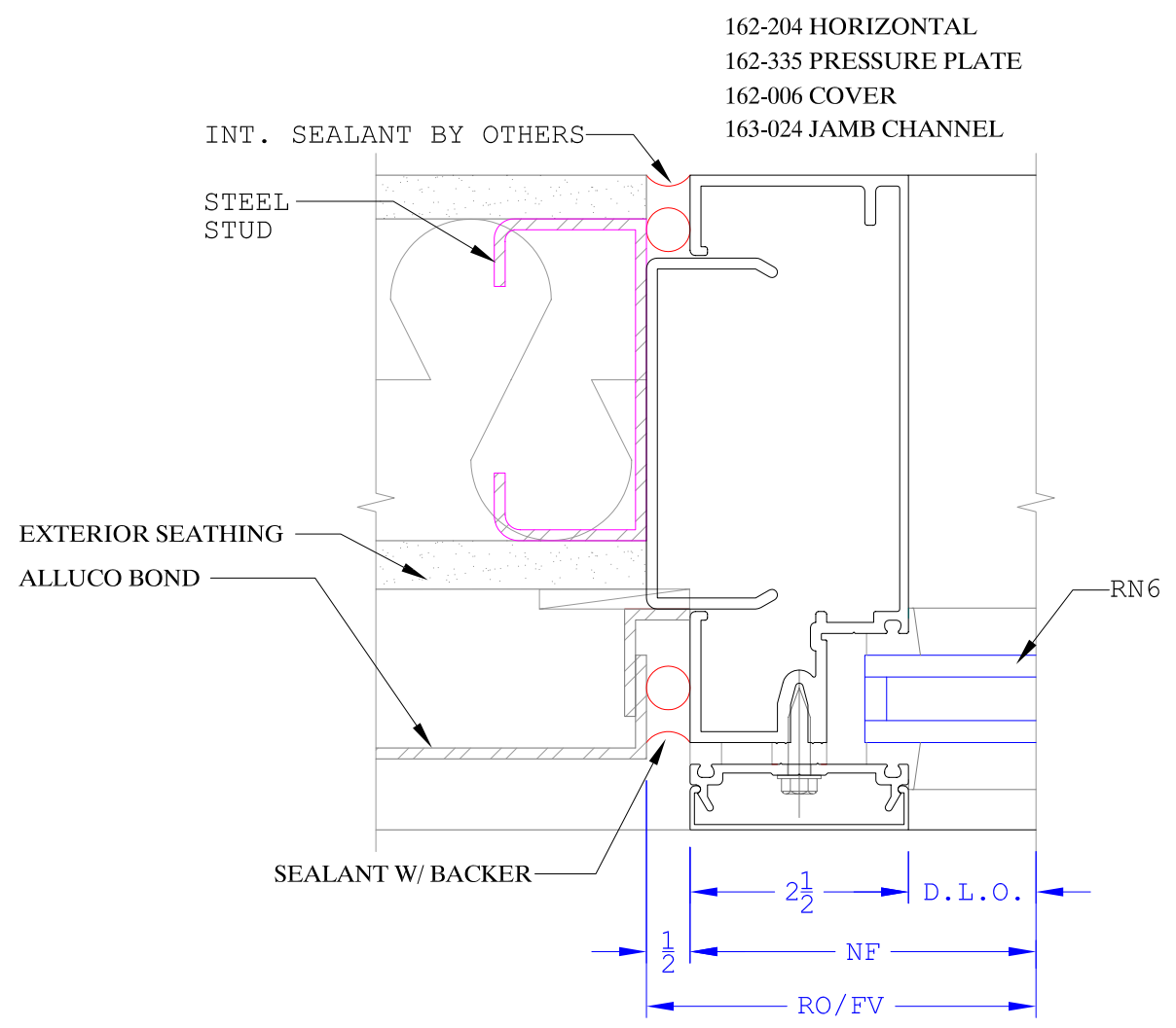
13 JAMB DETAIL ARCH. REF.: A4.1 ELEV. REF.: CW4, CW5
