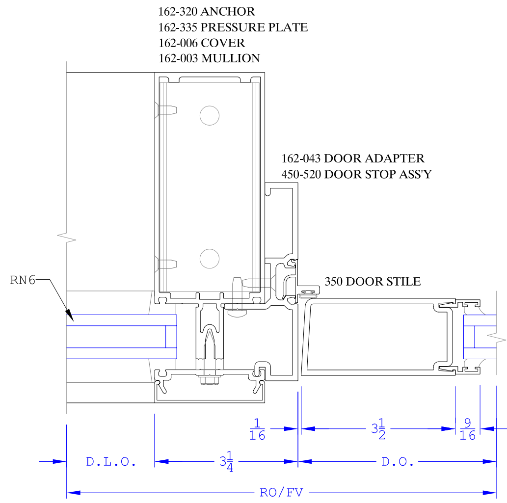
12 DOOR JAMB DETAIL ARCH. REF.: - ELEV. REF.: CW4
