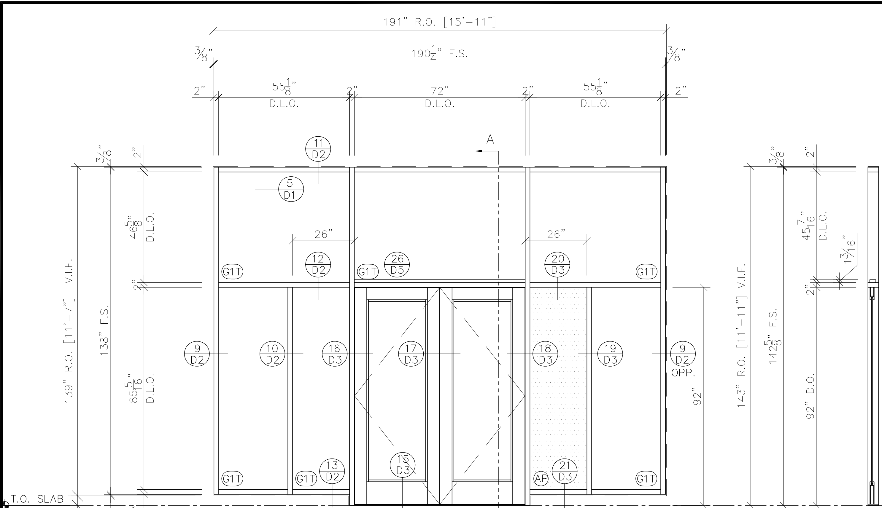
SECTION AA ARCH REF.: 1/A3.8
